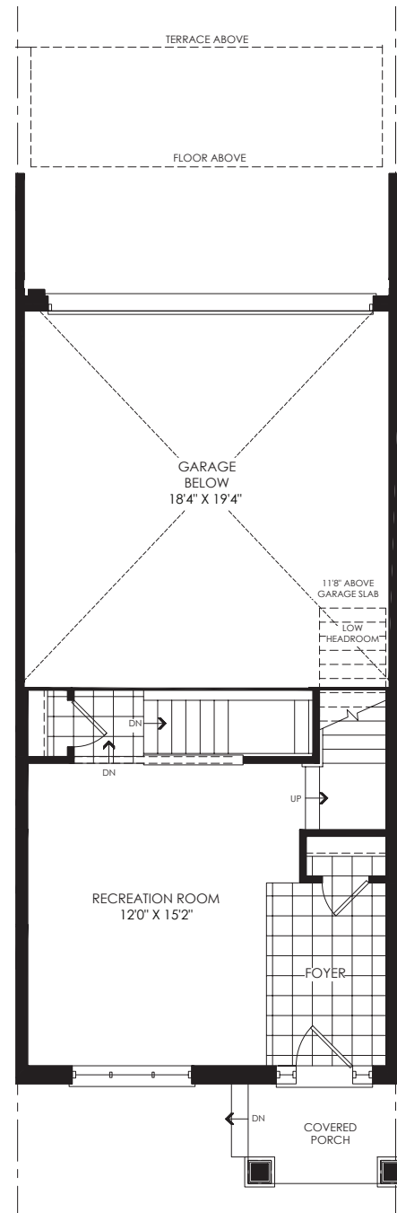
LOWER FLOOR
