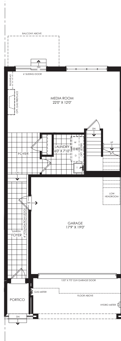
LOWER FLOOR
